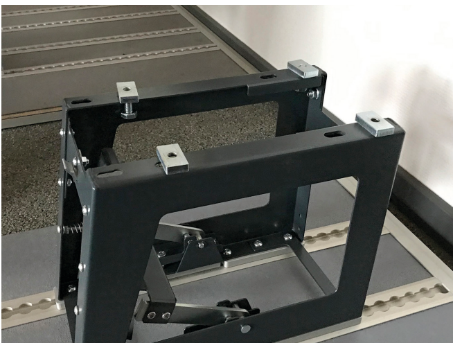
Place the 4 bolts on the leg
