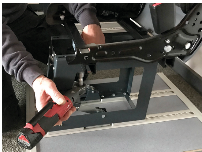
Tighten the bolts
